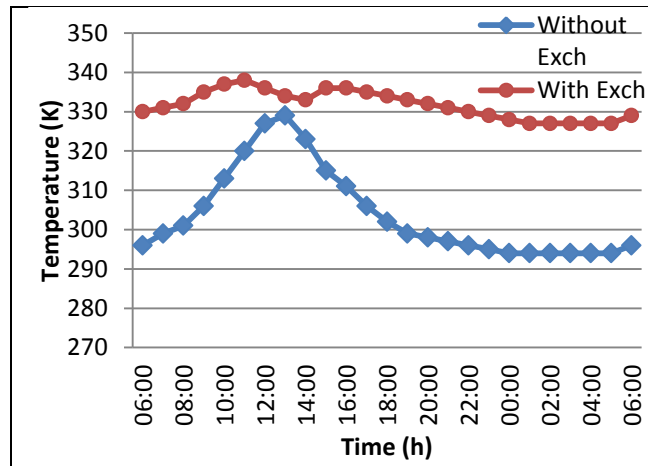
Figure 10 : Evolution of drying air temperature of solar dryer without and with breaking operating of heat exchanger from 11:00 till 15:00
