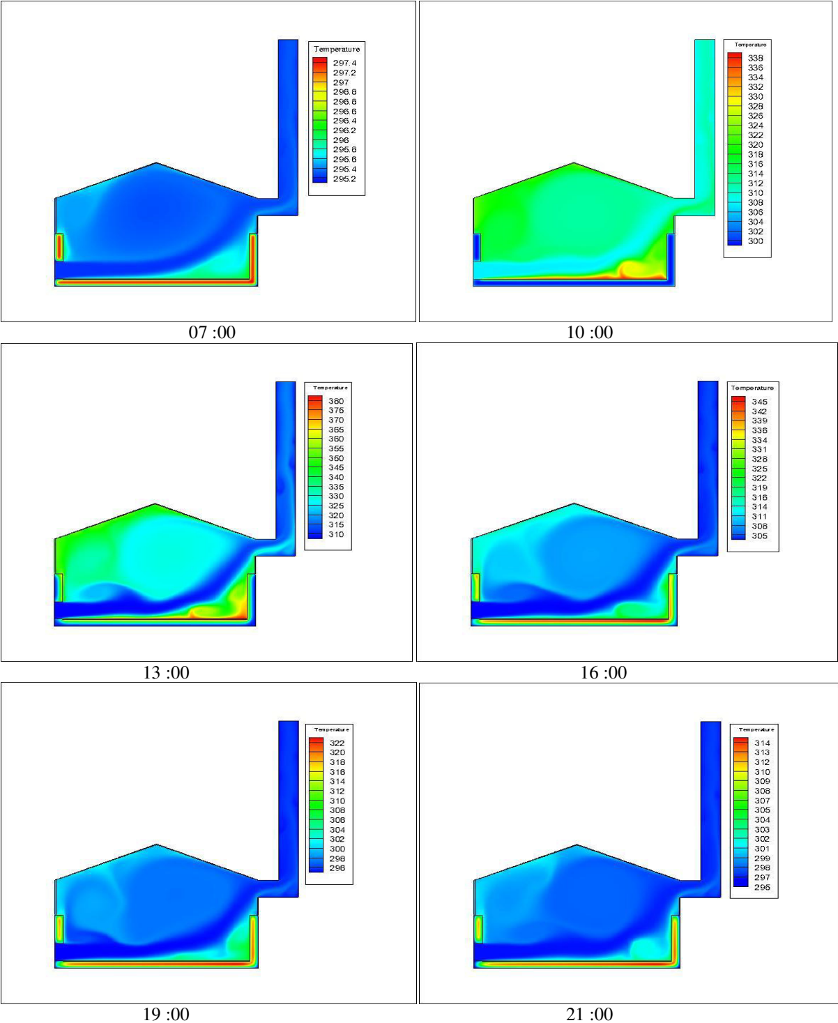
Figure 5: Evolution of temperature counter of solar dryer without heat exchanger
