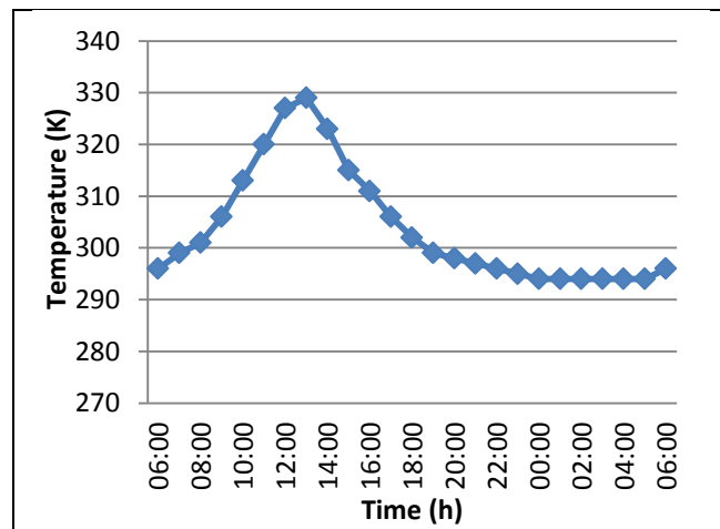
Figure 6: Evolution of the air temperature in the middle of the solar dryer without heat exchanger
