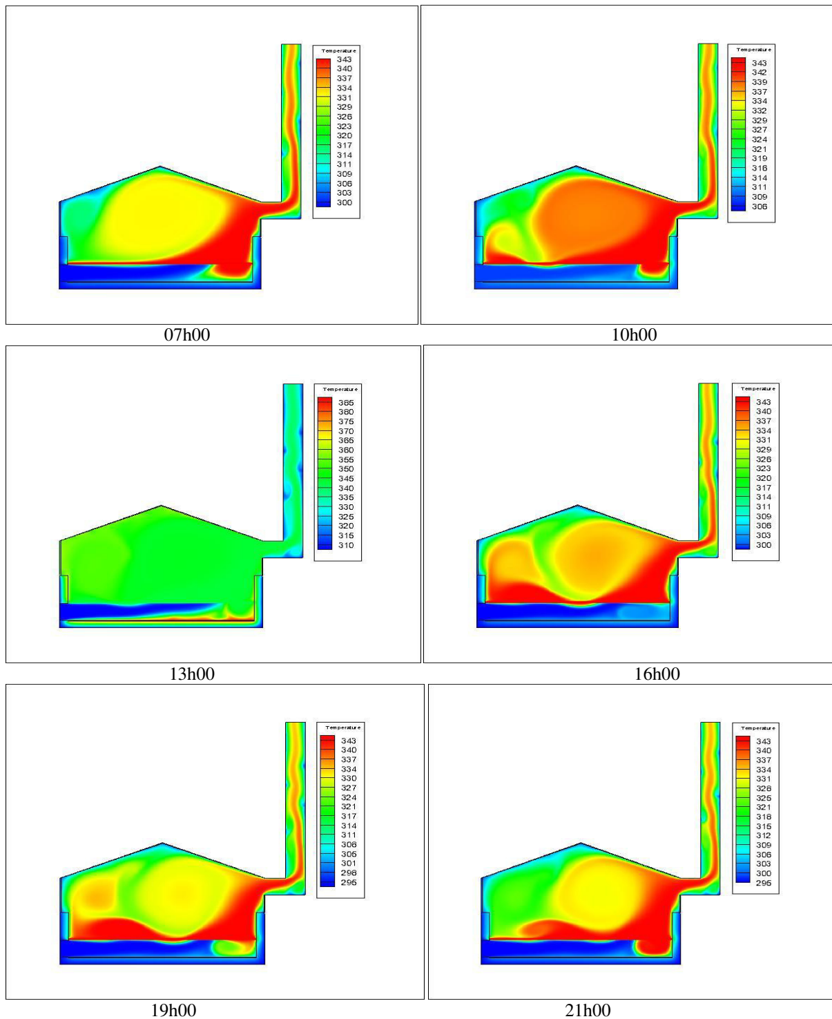
Figure 8 : Temperature fields in the solar dryer with heat exchanger
