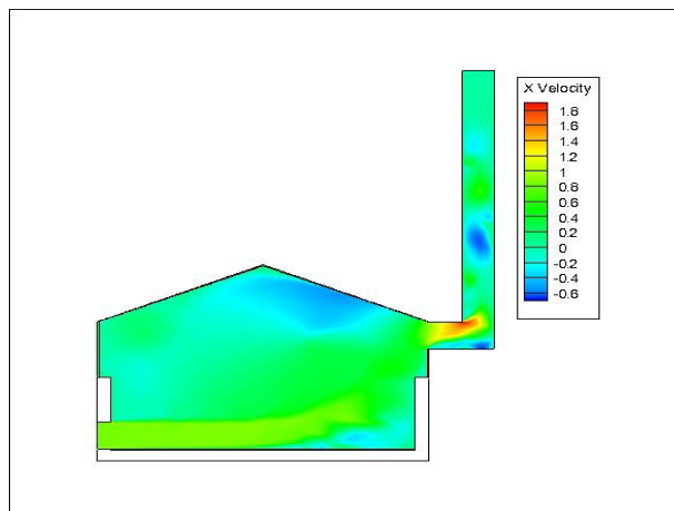
Figure 4: Contours of axial velocity of solar dryer without heat exchanger
