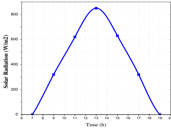
Figure 3: Variation of the solar radiation in function of time
