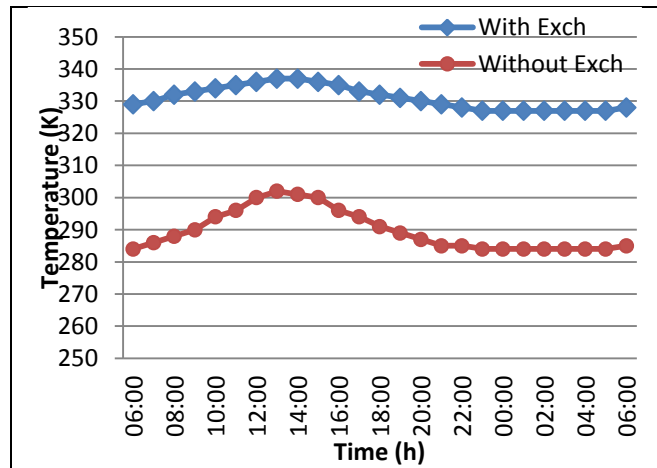
Figure 11 : Evolution of drying air temperature of solar dryer with and without heat exchanger at low solar radiation ( I=200\text{W/m}^2 )
