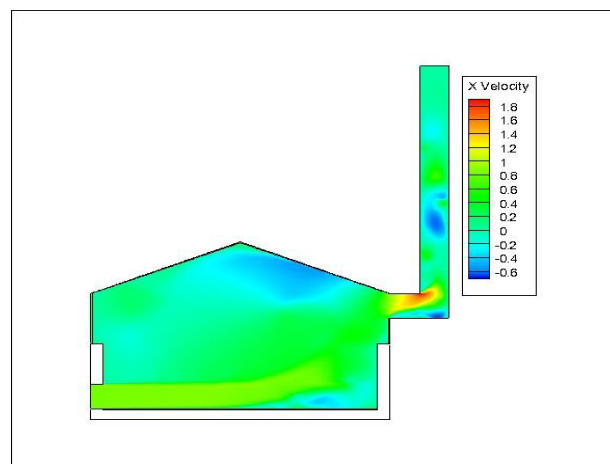
Figure 7 : Contours of axial velocity of solar dryer with integration of heat exchanger
