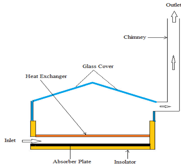
Figure 1: Direct solar dryer with integrated heat exchanger
