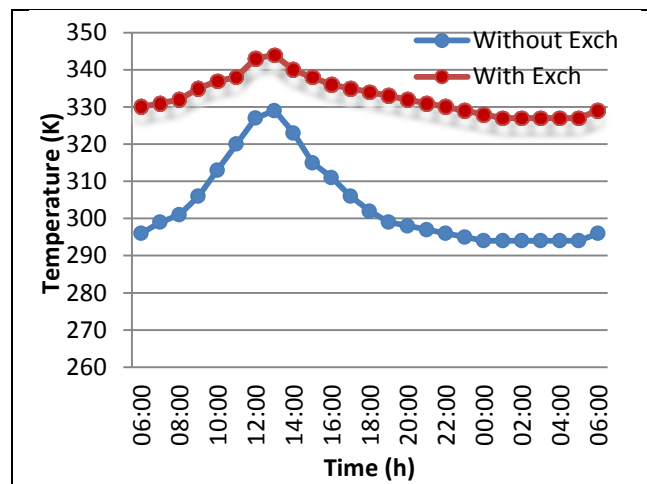
Figure 9 : Evolution of drying air temperature of solar dryer with and without heat exchanger
